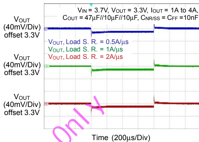
Load Transient Response vs. Load Slew Rate
