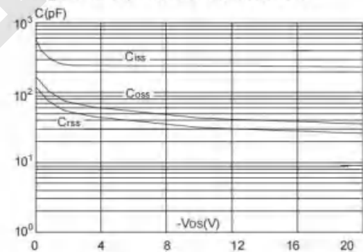
Figure 6: Capacitance Characteristics
